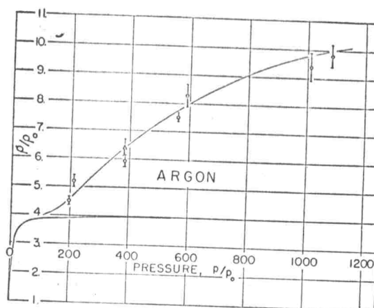
FIG. 1. Hugoniot of Argon (initial conditions, T_0 = 27^\circ\text{C} , P_0 = .80 \times 10^8 dynes/cm 2 ). The point shown by the triangle is for a mixture of 93 percent argon, 7 percent oxygen.
